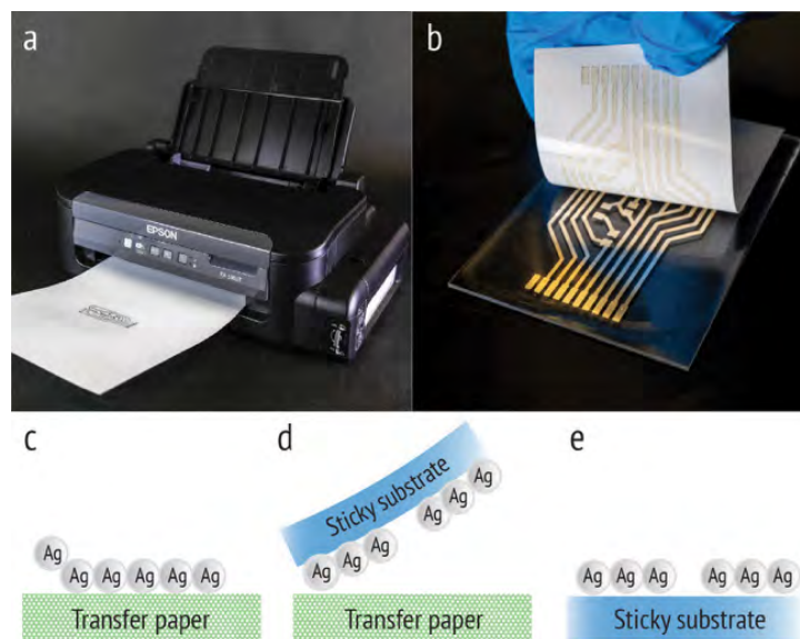
Fig. 2. Overview of Silver Tape. Conductive patterns are (a) printed on transfer paper, (b) peeled off and transferred by hand. (c-e) Schematics of the transfer process of silver nanoparticles from transfer paper to a sticky substrate.
