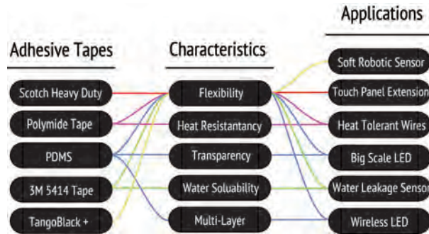
Fig. 8. Application Overview
